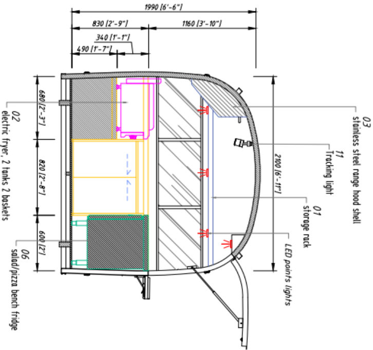
FOOD TRUCK SECTION_3-3
